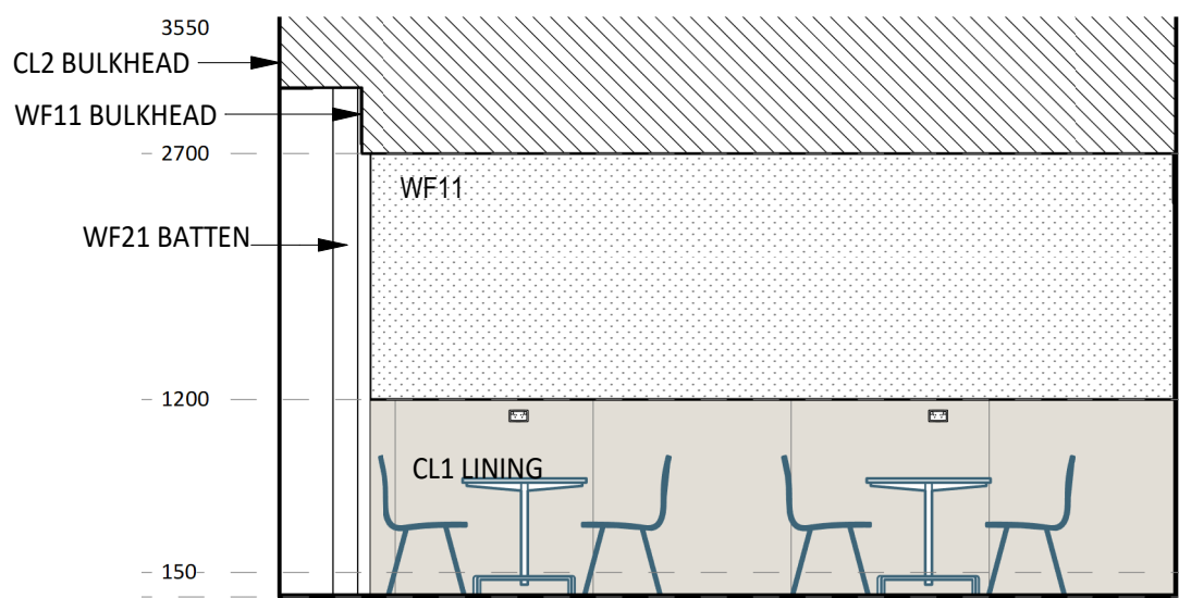
4 ELEVATION DETAIL 60-037 1 : 50
