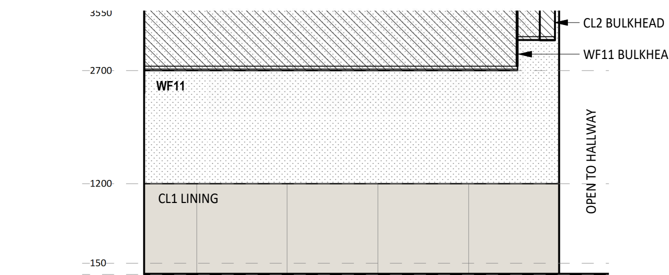
5 ELEVATION DETAIL 60-011 1 : 50
